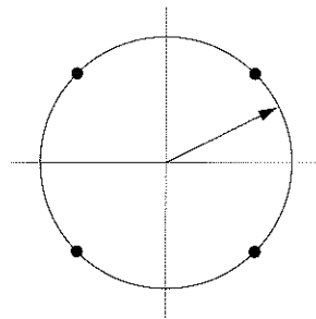
The relaxation of the constraint allows \mathbf{s} to point to any position on a hypersphere circumscribing the original hypercube, rather than just the corners of the hypercube.
