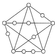
An expansion of K_5 .
