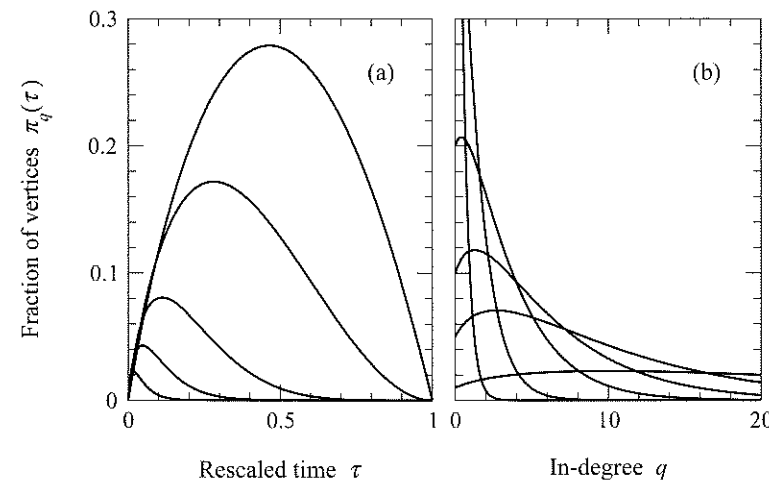
Figure 14.3: Distribution of vertices in Price's model as a function of in-degree and time of creation. The two panels show the distribution \pi_q(\tau) , Eq. (14.57), for c = 3 and a = 1.5 as (a) a function of \tau for (top to bottom) q = 1, 2, 5, 10 , and 20 , and (b) a function of q for \tau = 0.01 (flattest curve), 0.05, 0.1, 0.5 , and 0.9 (steepest curve).
