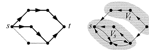
Figure 10.9: Finding a minimum cut set. Once we have found a set of maximum flows for a given s and t (left) we can find a corresponding minimum cut set by considering the residual graph (right). The set V_s is the set of vertices reachable from s by following directed edges on the residual graph and V_t is the rest of the vertices. The minimum cut set is the set of edges (two of them in this case) that connect V_s to V_t on the original network.
