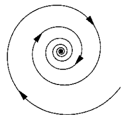
The flows around a fixed point whose Jacobian matrix has complex eigenvalues describe a spiral.
