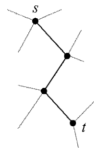
A network path from s to t of length d (where d = 3 in this case) necessarily includes a path of length d - 1 (i.e., 2) from s to an immediate neighbor of t .
