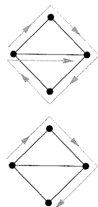
Examples of Eulerian and Hamiltonian paths in a small network.
