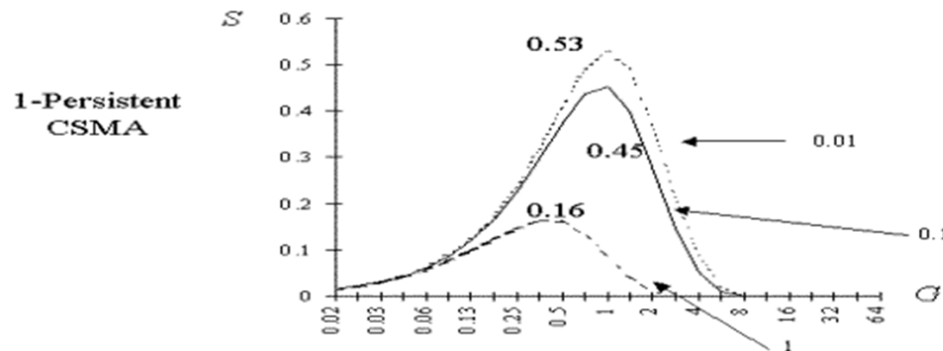
Throughput of 1-persistent CSMA
