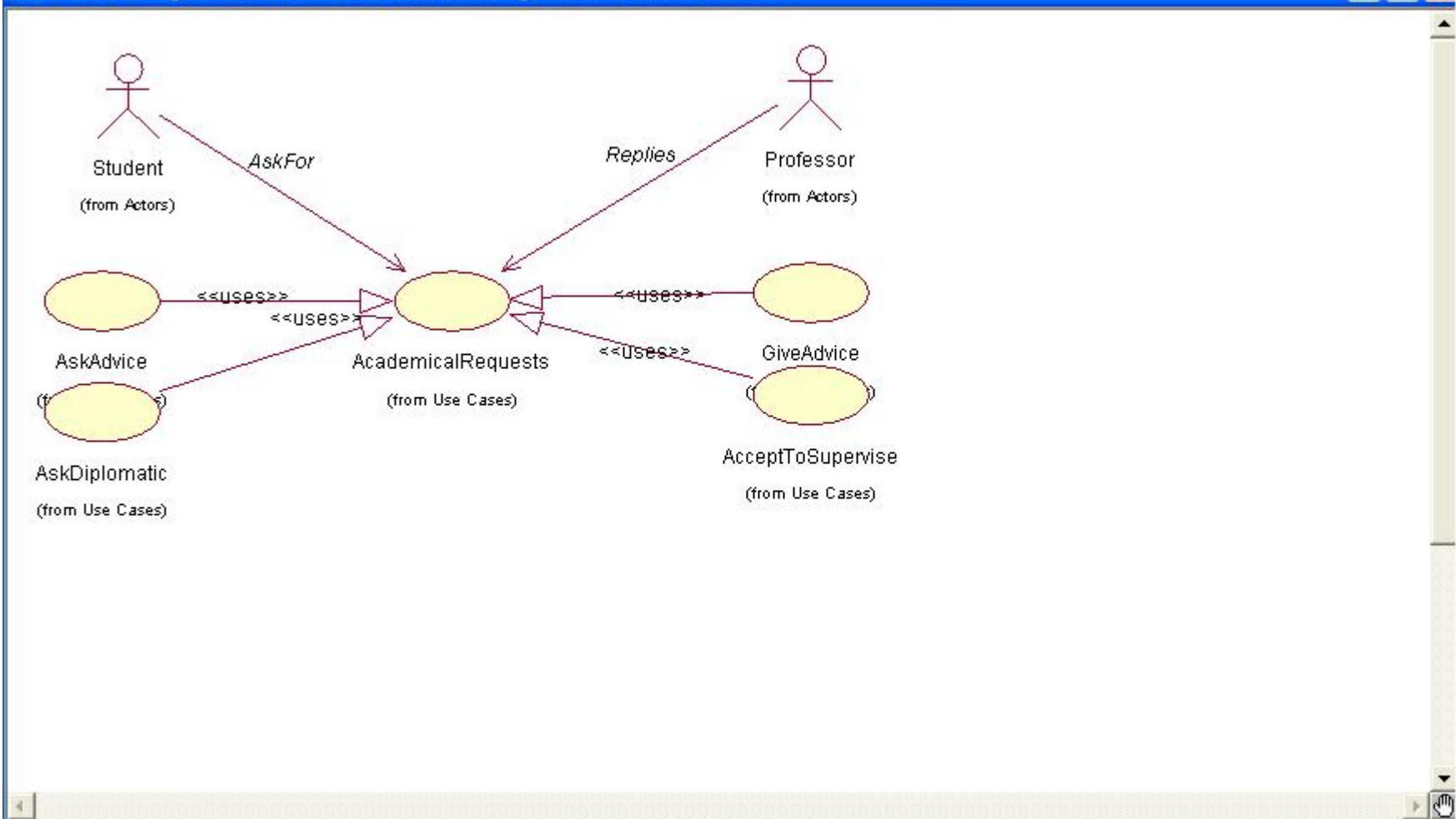
Use Case Diagram: Use Case View / UseCaseDiagramKatsionisAcademical
