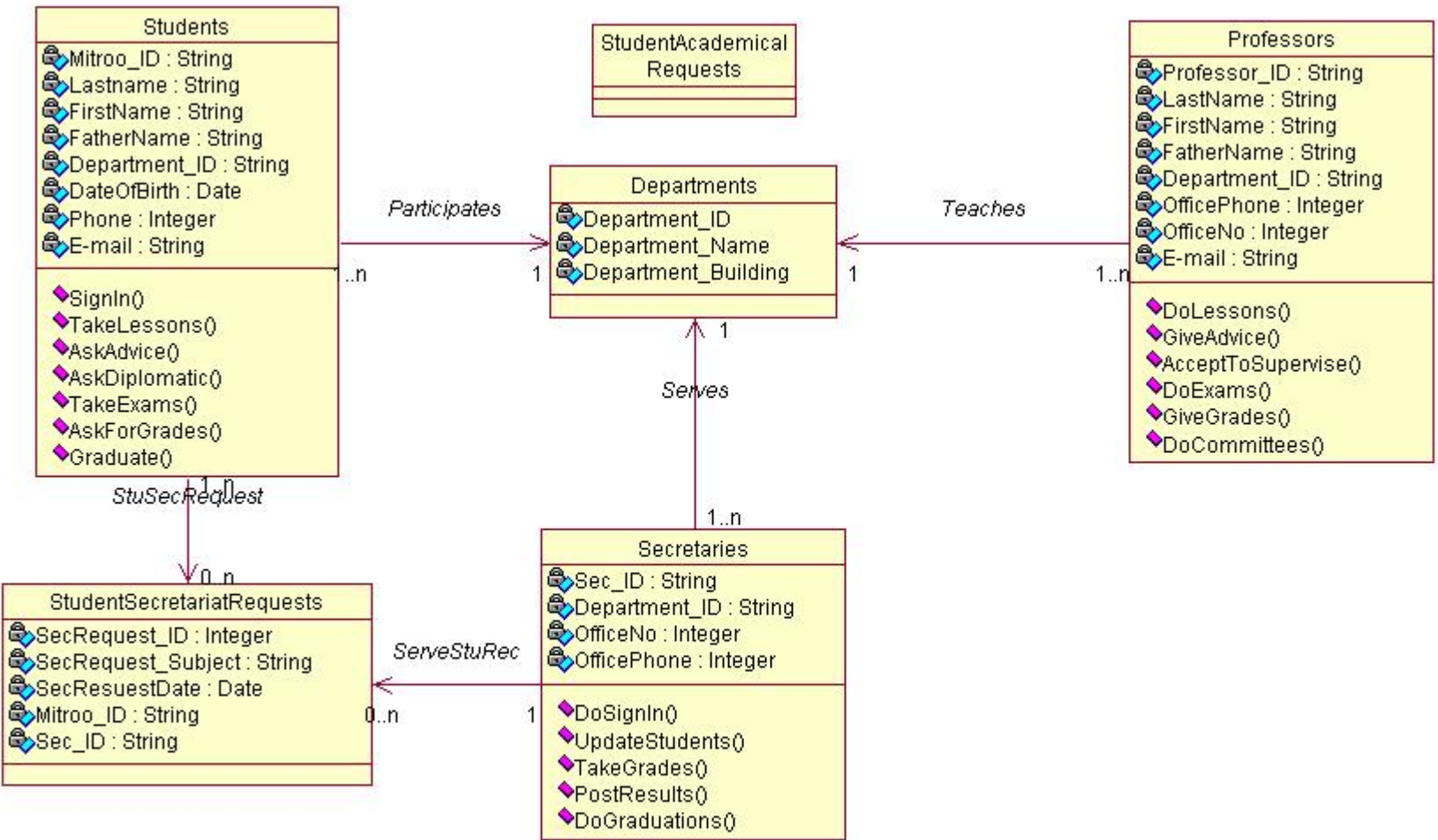
Class Diagram: Logical View / ClassDiagramKatsionis
