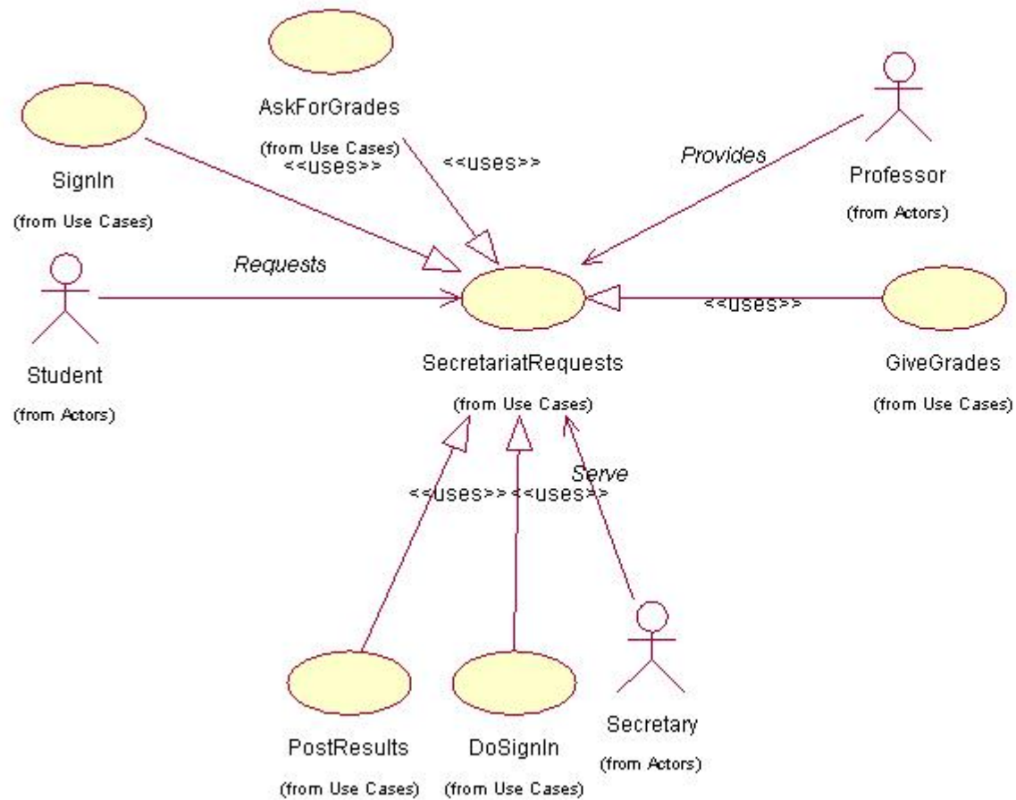
Use Case Diagram: Use Case View / UseCaseDiagramKatsionisSecretariat
