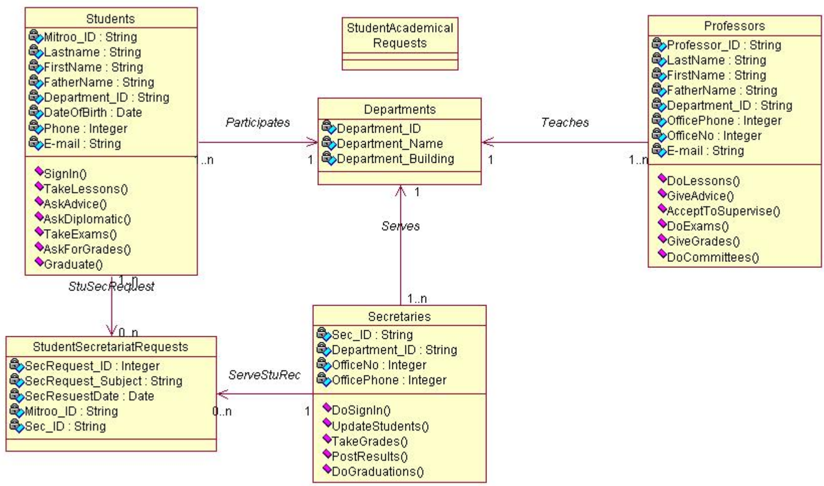
Class Diagram: Logical View / ClassDiagramKatsionis
