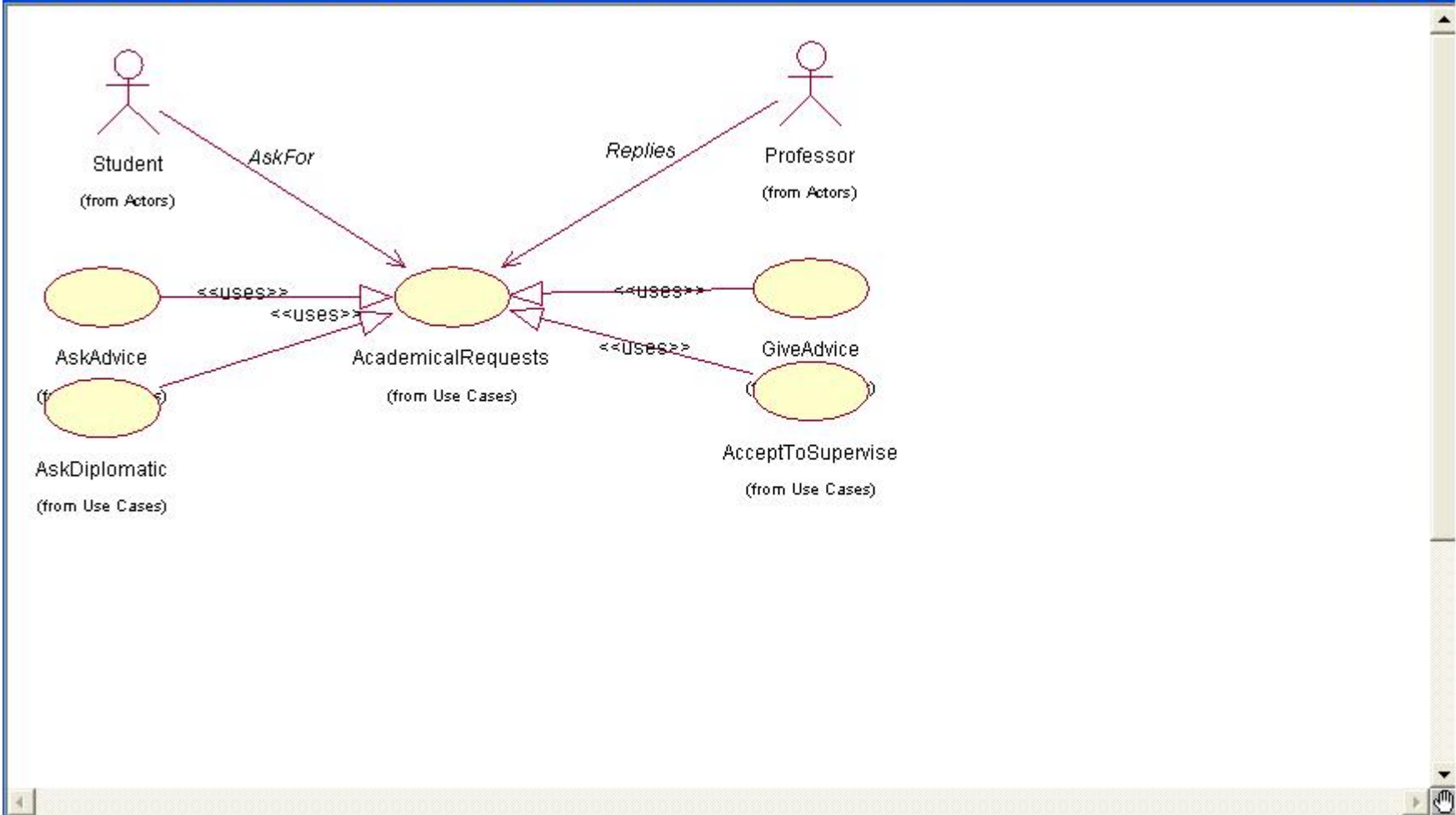
Use Case Diagram: Use Case View / UseCaseDiagramKatsionisAcademical
