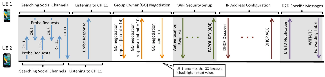
Fig. 8. D2D device discovery and connection establishment procedure.
