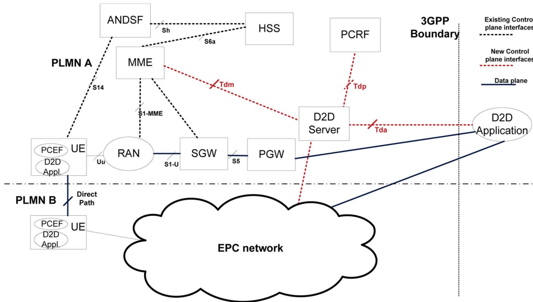
Fig. 7. Illustration of proposed D2D architecture in [101].
