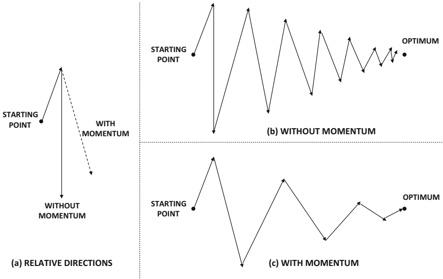
Figure 3.11: Effect of momentum in smoothing zigzag updates
