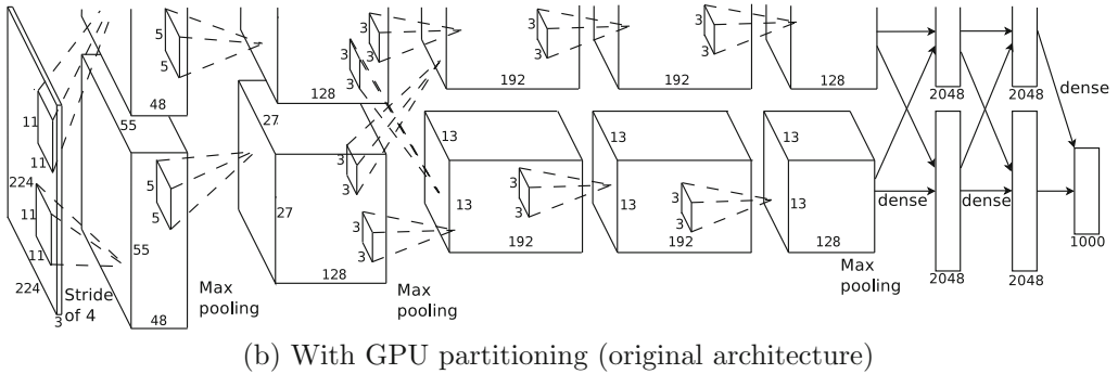
Figure 8.9: The AlexNet architecture. The ReLU activations follow each convolution layer, and are not explicitly shown. Note that the max-pooling layers are labeled as MP, and they follow only a subset of the convolution-ReLU combination layers. The architectural diagram in (b) is from [A. Krizhevsky, I. Sutskever, and G. Hinton. Imagenet classification with deep convolutional neural networks. NIPS Conference , pp. 1097–1105. 2012.] ©2012 A. Krizhevsky, I. Sutskever, and G. Hinton.
