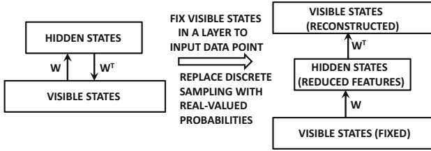
(b) Discrete graphical model to approximate real-valued neural network
