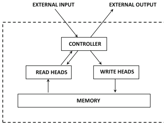
Figure 10.6: The neural Turing machine
