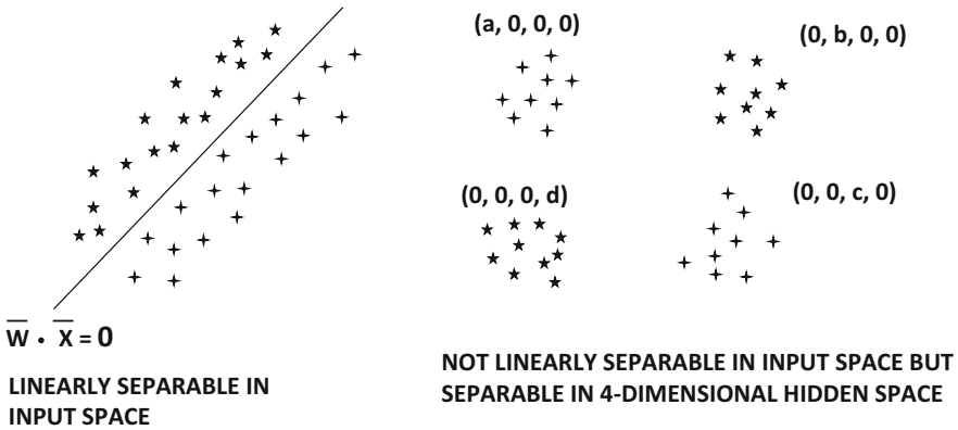
Figure 5.2: Revisiting Figure 1.4: The Gaussian RBF promotes separability because of the transformation to the hidden layer.
