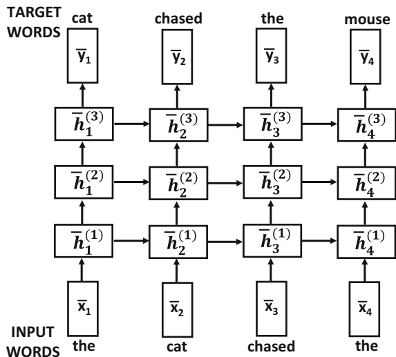
Figure 7.6: Multi-layer recurrent neural networks
