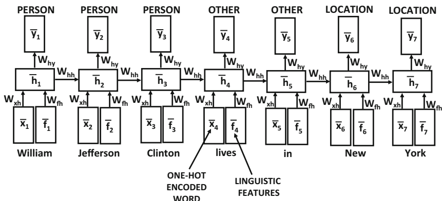
Figure 7.12: Token-wise classification with linguistic features
