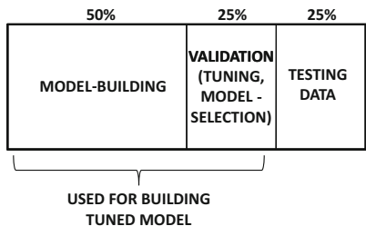
Figure 4.4: Partitioning a labeled data set for evaluation design
