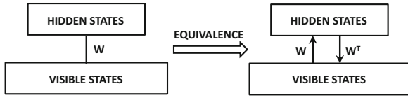
(a) Equivalence of directed and undirected relationships
