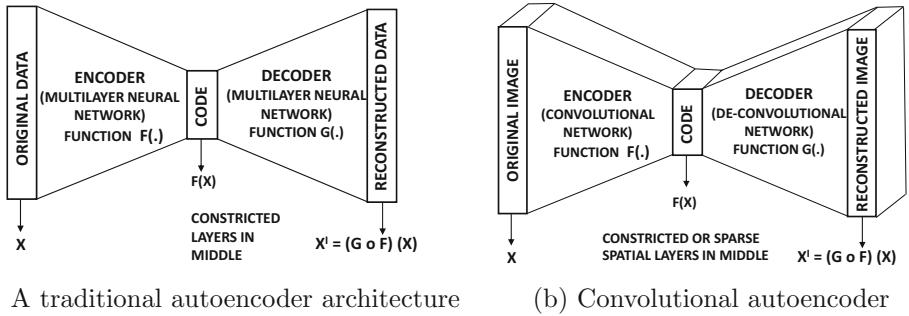
Figure 8.17: A traditional autoencoder and a convolutional autoencoder.
