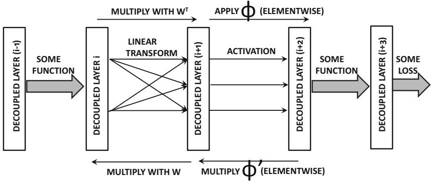
Figure 3.7: A decoupled view of backpropagation
