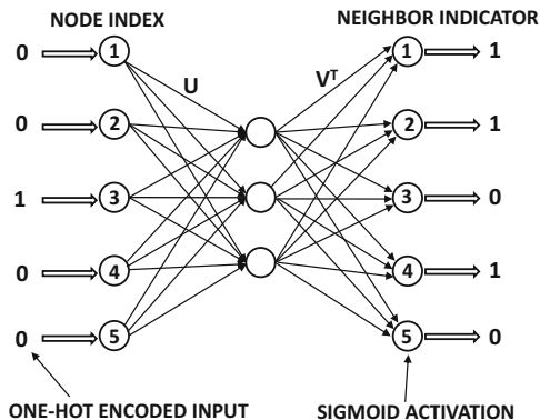
Figure 2.17: A graph of five nodes is shown together with a neural architecture for row index to neighbor indicator mapping. The shown input and output represent node 3 and its neighbors. Note the similarity to Figure 2.13. The main difference is that there are no missing values above, and the number of inputs is the same as the number of outputs for a square matrix. Both input and outputs are binary vectors. However, if negative sampling is used with sigmoid activation, most output nodes with zero values may be dropped.
