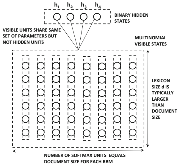
Figure 6.8: The RBM for each document is illustrated. The number of visible units is equal to the number of words in each document
