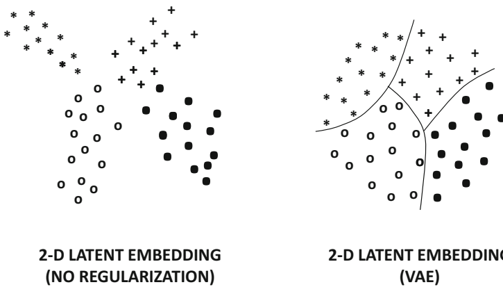
Figure 4.14: Illustrations of the embeddings created by a variational autoencoder in relation to the unregularized version. The unregularized version has large discontinuities in the latent space, which might not correspond to meaningful points. The Gaussian embedding of the points in the variational autoencoder makes sampling possible.
